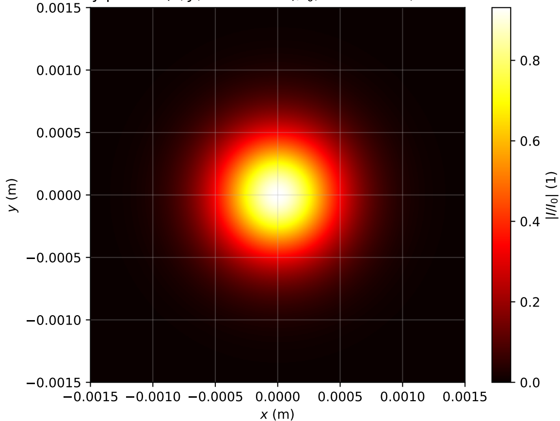
Intensity profile I(x, y, z = 1.274m)/I_0 , Pin=0.4Pcr, artificial time
